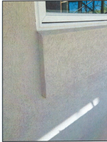
Views of the completed EIFS finish system with copper flashing and sealants applied.
